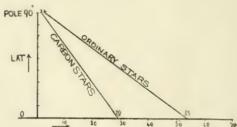
FIG. 38.—Comparison of relative numbers of stars generally and carbon stars.
